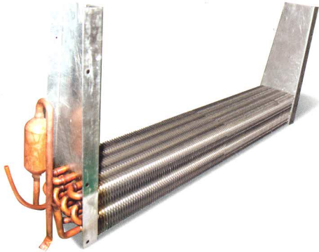
Evaporator for visi cooler/upright freezer
